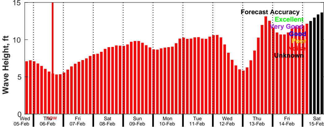
CMEMS Wave Forecast for NDBC 46053 from 05-Feb-2025 17:00:00 to 15-Feb-2025 17:00:00
