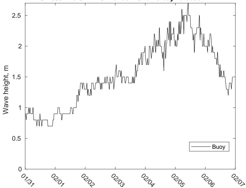
NDBC 46054 vs CMEMS Waves: 10 to 16 day forecast
