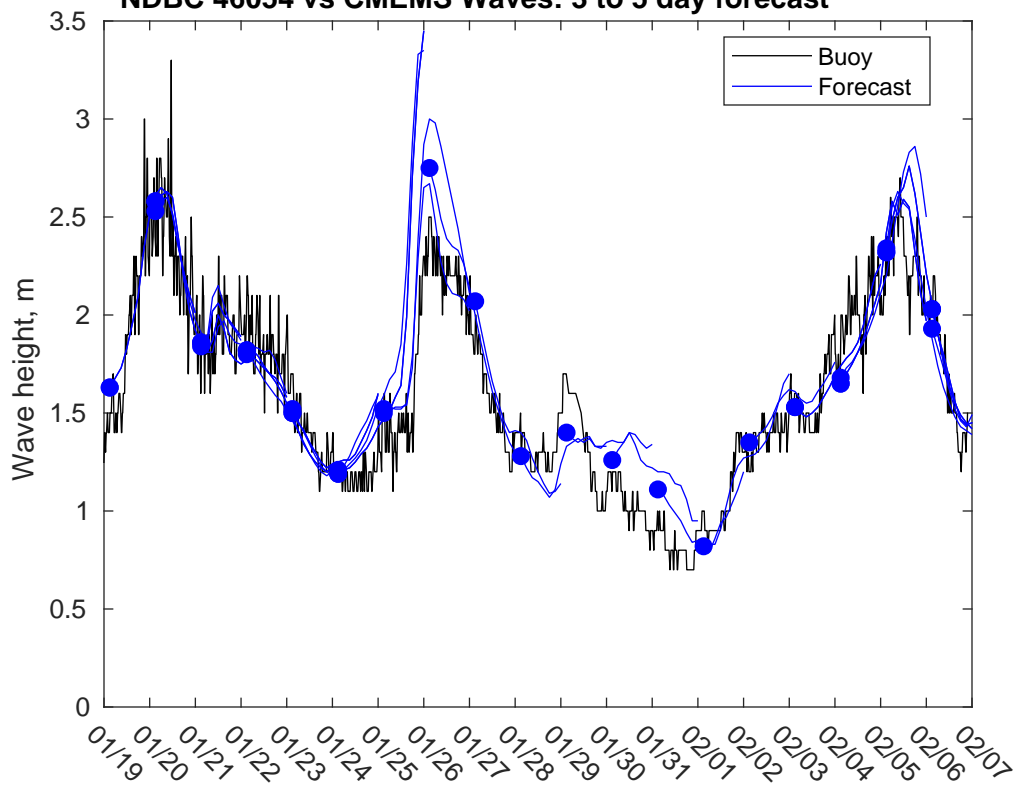
NDBC 46054 vs CMEMS Waves: 3 to 5 day forecast
