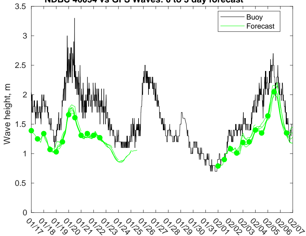
NDBC 46054 vs GFS Waves: 0 to 3 day forecast
