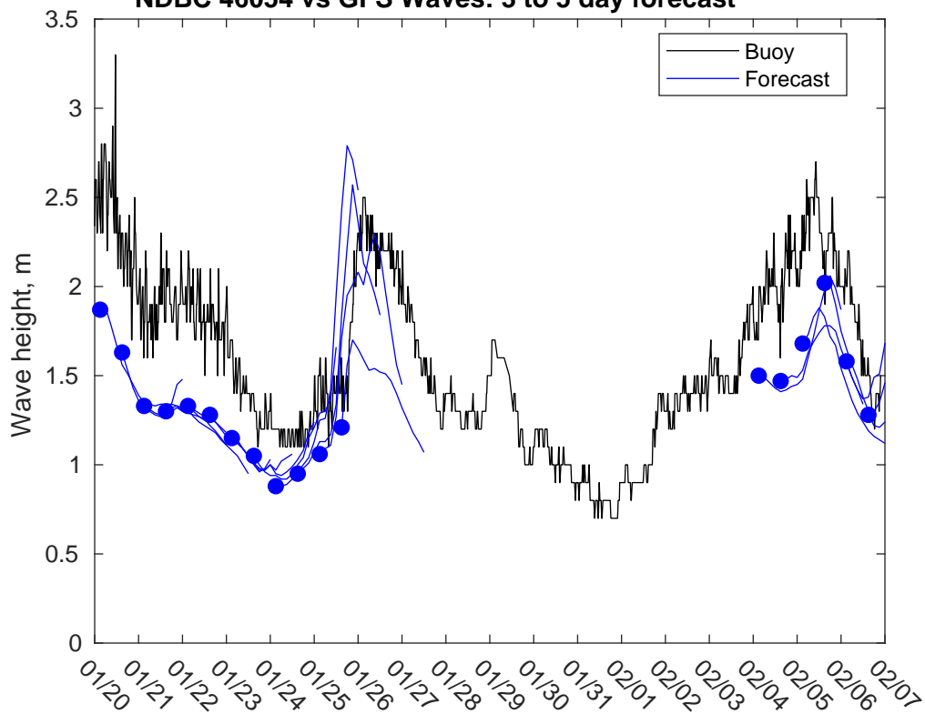
NDBC 46054 vs GFS Waves: 3 to 5 day forecast
