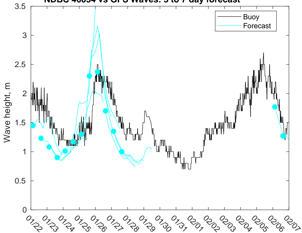
NDBC 46054 vs GFS Waves: 5 to 7 day forecast
