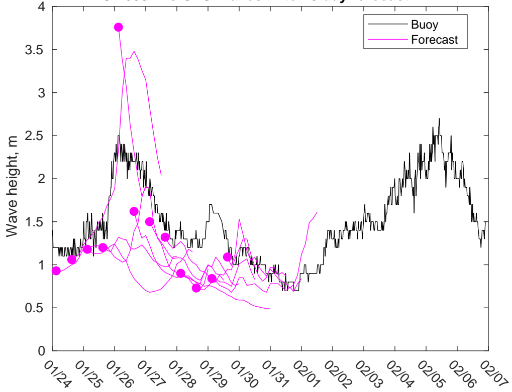
NDBC 46054 vs GFS Waves: 7 to 10 day forecast
