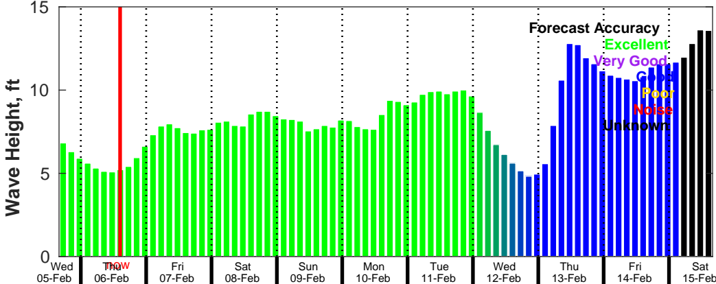
CMEMS Wave Forecast for NDBC 46054 from 05-Feb-2025 16:00:00 to 15-Feb-2025 16:00:00
