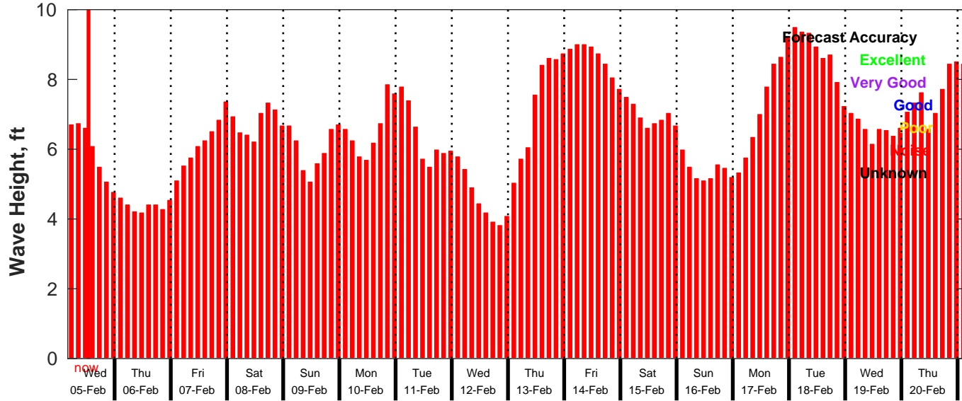
GFS Wave Forecast for NDBC 46054 from 05-Feb-2025 04:00:00 to 21-Feb-2025 04:00:00
