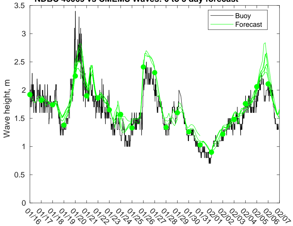
NDBC 46069 vs CMEMS Waves: 0 to 3 day forecast
