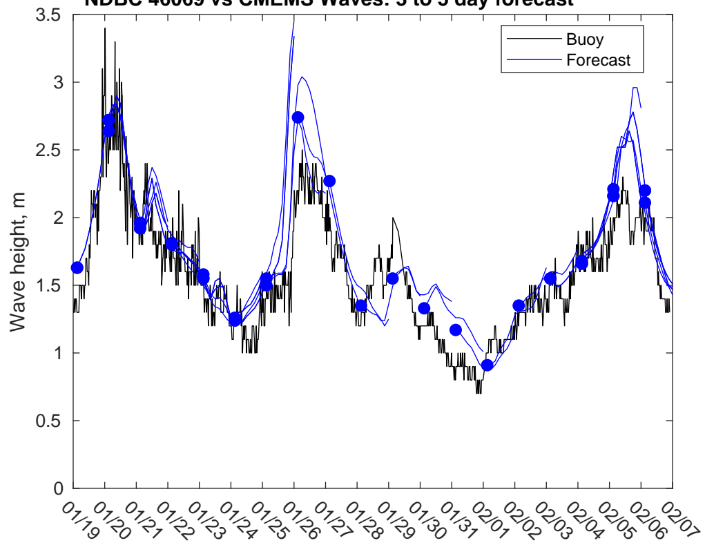
NDBC 46069 vs CMEMS Waves: 3 to 5 day forecast
