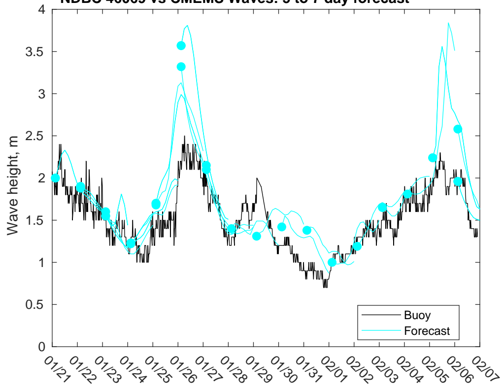
NDBC 46069 vs CMEMS Waves: 5 to 7 day forecast
