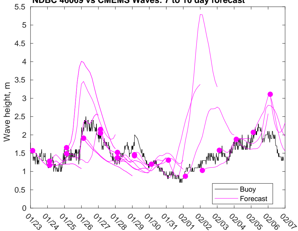
NDBC 46069 vs CMEMS Waves: 7 to 10 day forecast
