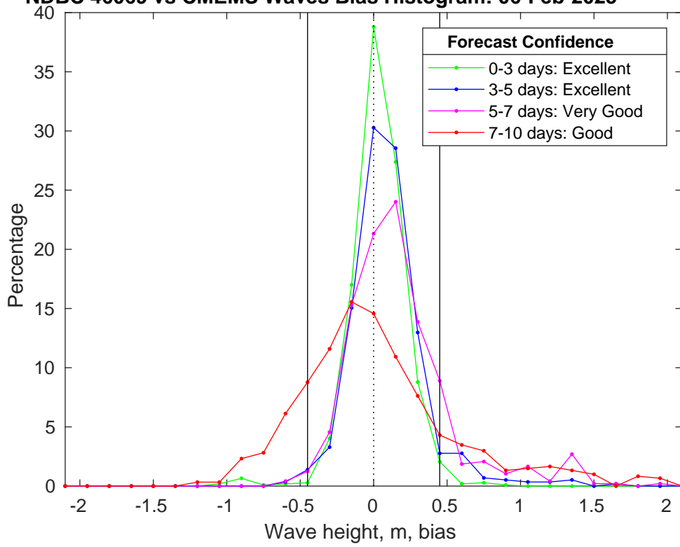
NDBC 46069 vs CMEMS Waves Bias Histogram: 06-Feb-2025
