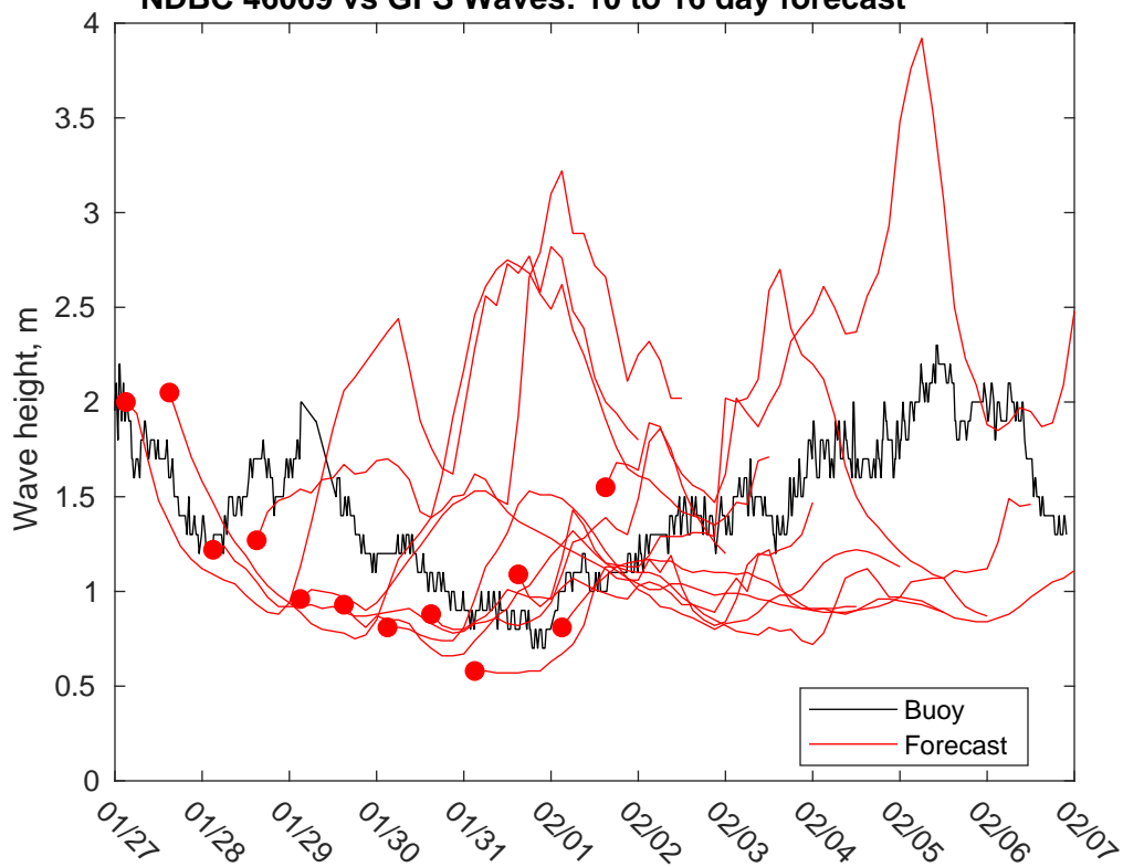
NDBC 46069 vs GFS Waves: 10 to 16 day forecast
