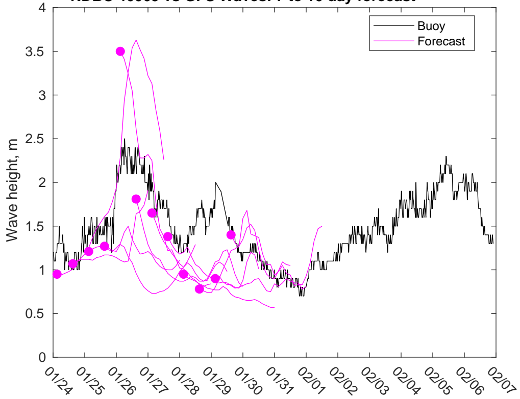
NDBC 46069 vs GFS Waves: 7 to 10 day forecast
