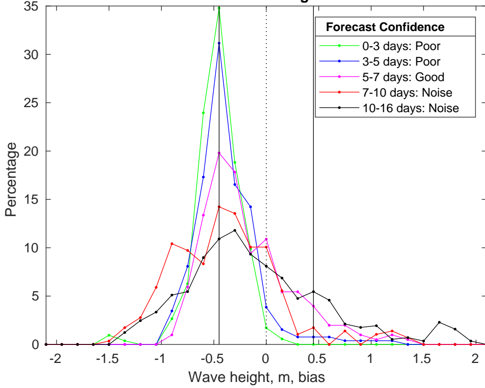
NDBC 46069 vs GFS Waves Bias Histogram: 06-Feb-2025
