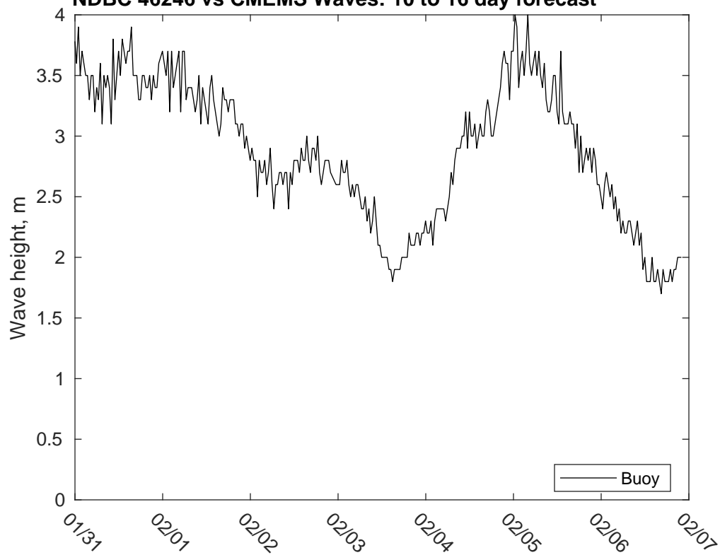
NDBC 46246 vs CMEMS Waves: 10 to 16 day forecast
