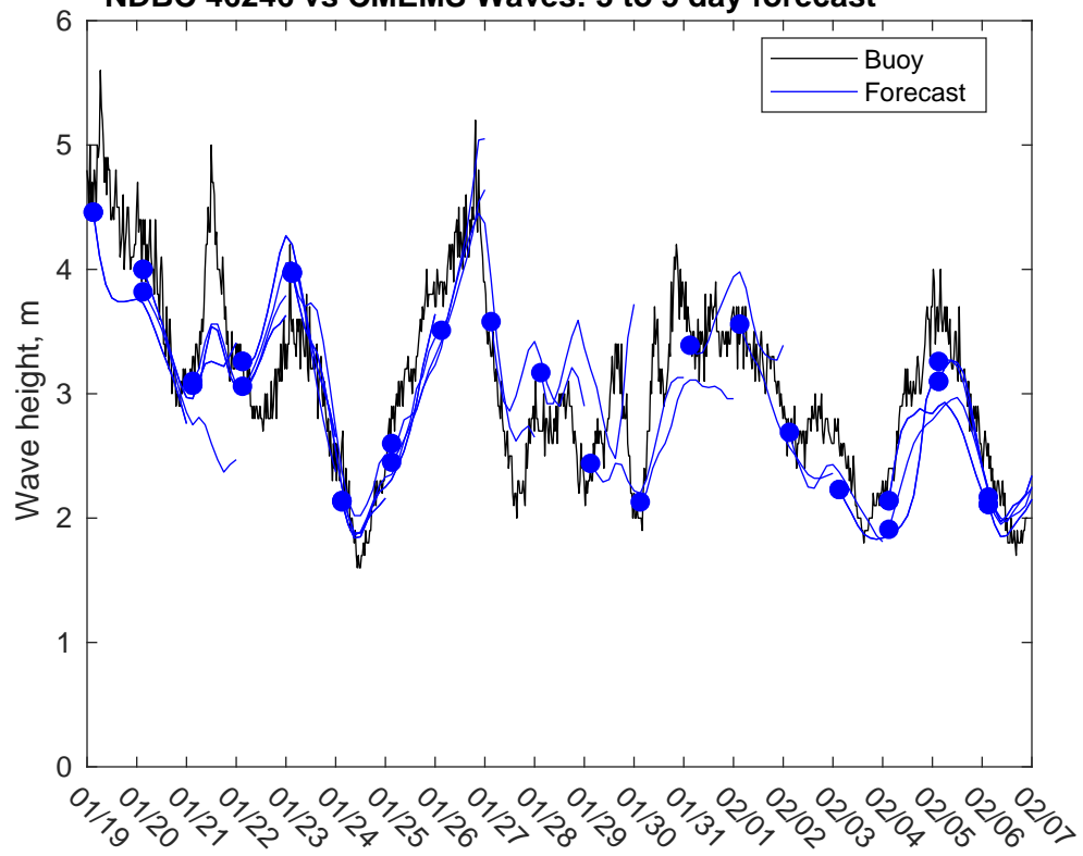
NDBC 46246 vs CMEMS Waves: 3 to 5 day forecast
