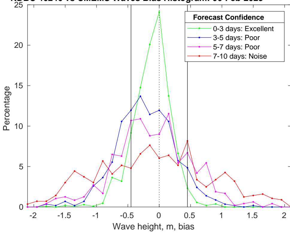
NDBC 46246 vs CMEMS Waves Bias Histogram: 06-Feb-2025
