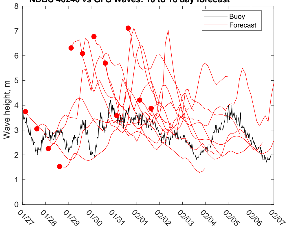
NDBC 46246 vs GFS Waves: 10 to 16 day forecast
