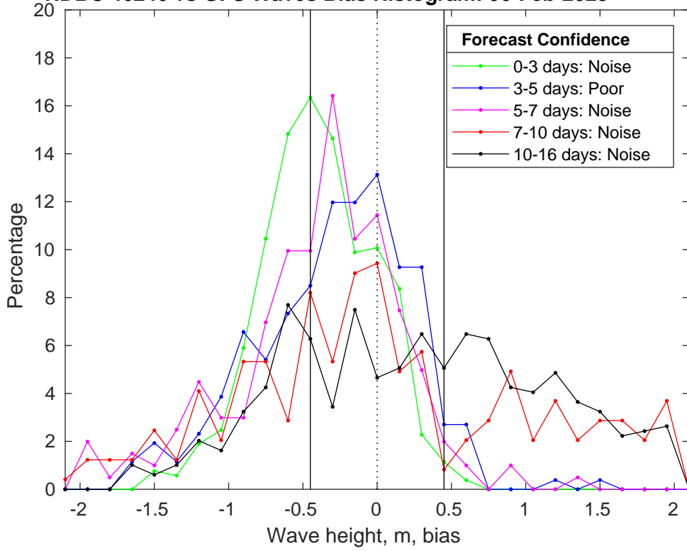
NDBC 46246 vs GFS Waves Bias Histogram: 06-Feb-2025
