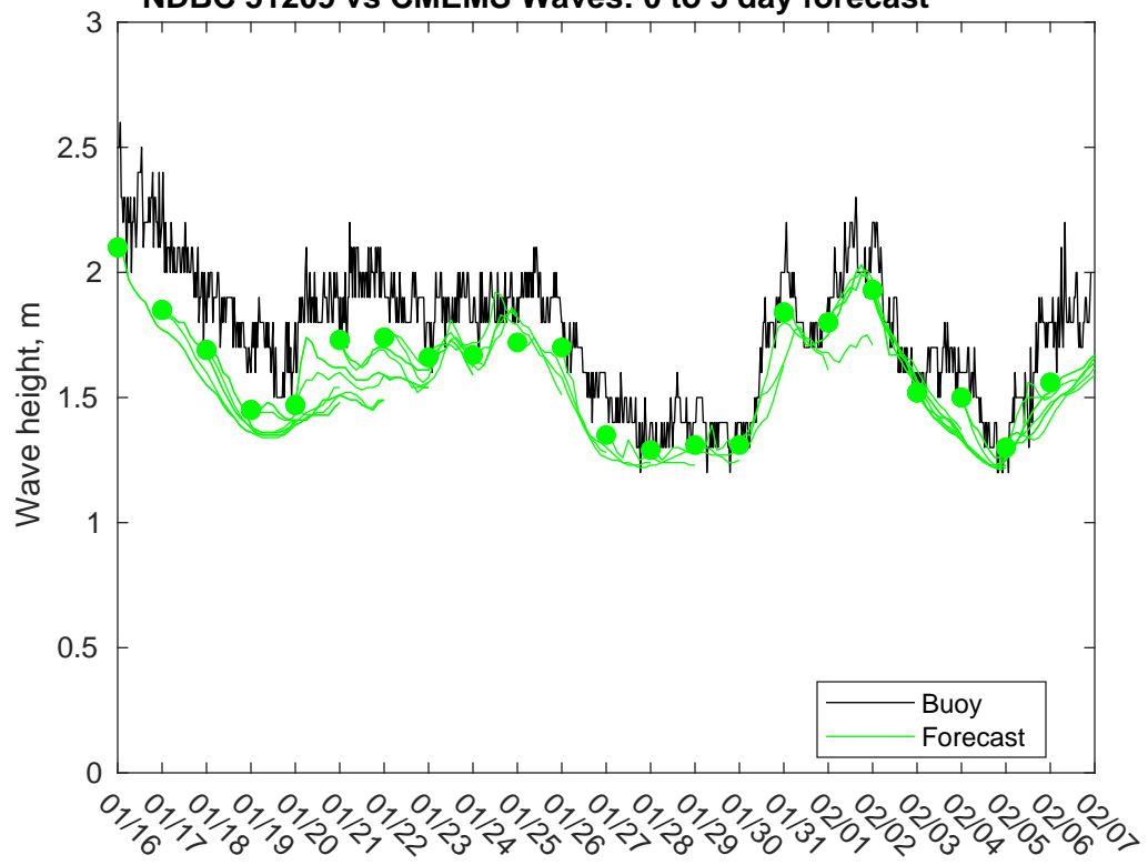
NDBC 51209 vs CMEMS Waves: 0 to 3 day forecast
