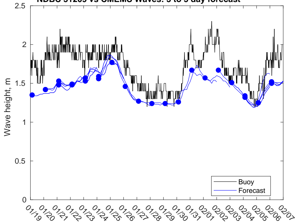
NDBC 51209 vs CMEMS Waves: 3 to 5 day forecast
