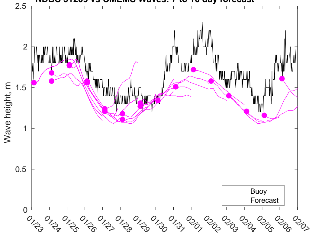
NDBC 51209 vs CMEMS Waves: 7 to 10 day forecast
