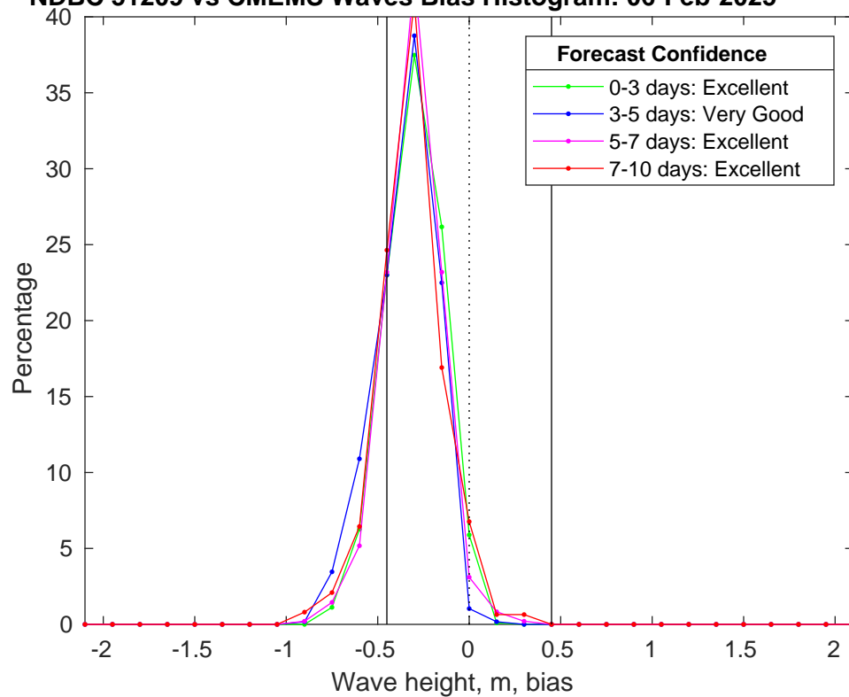
NDBC 51209 vs CMEMS Waves Bias Histogram: 06-Feb-2025
