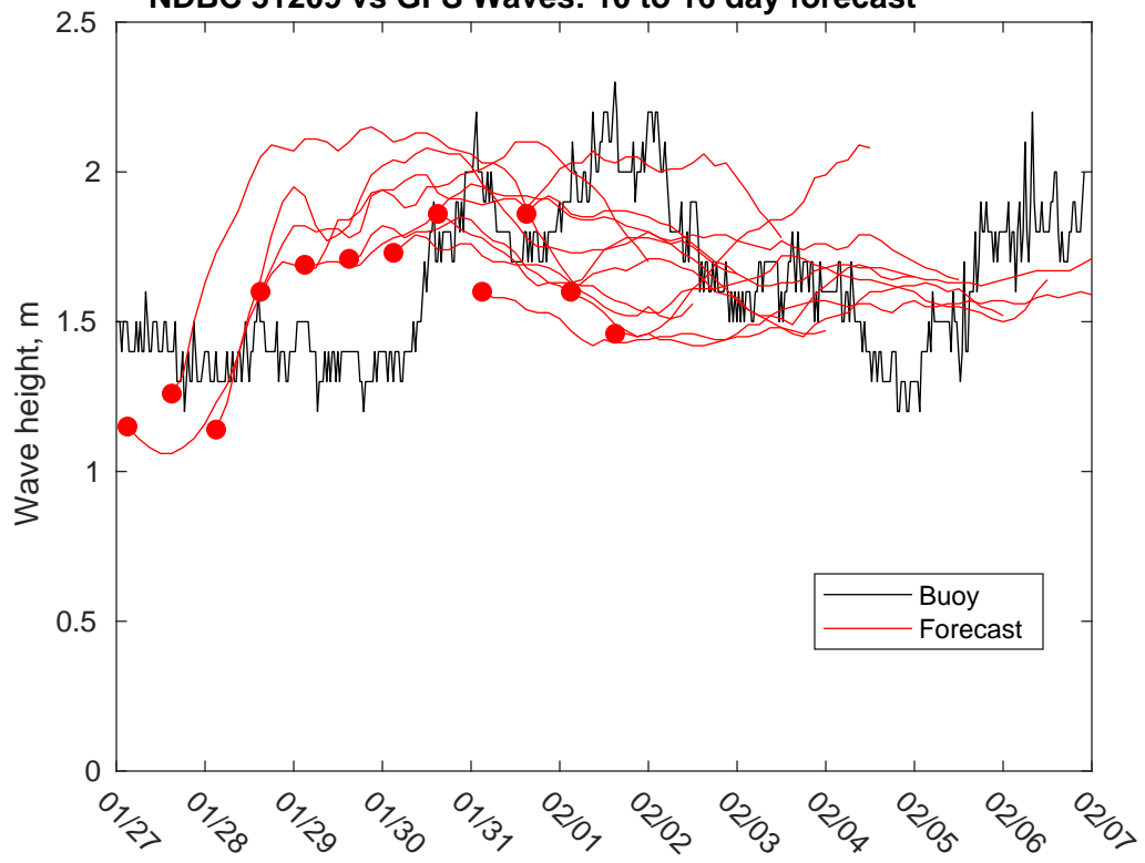
NDBC 51209 vs GFS Waves: 10 to 16 day forecast
