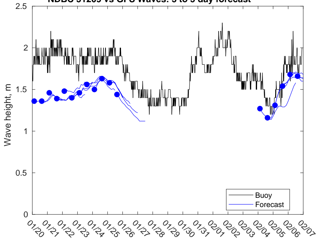
NDBC 51209 vs GFS Waves: 3 to 5 day forecast
