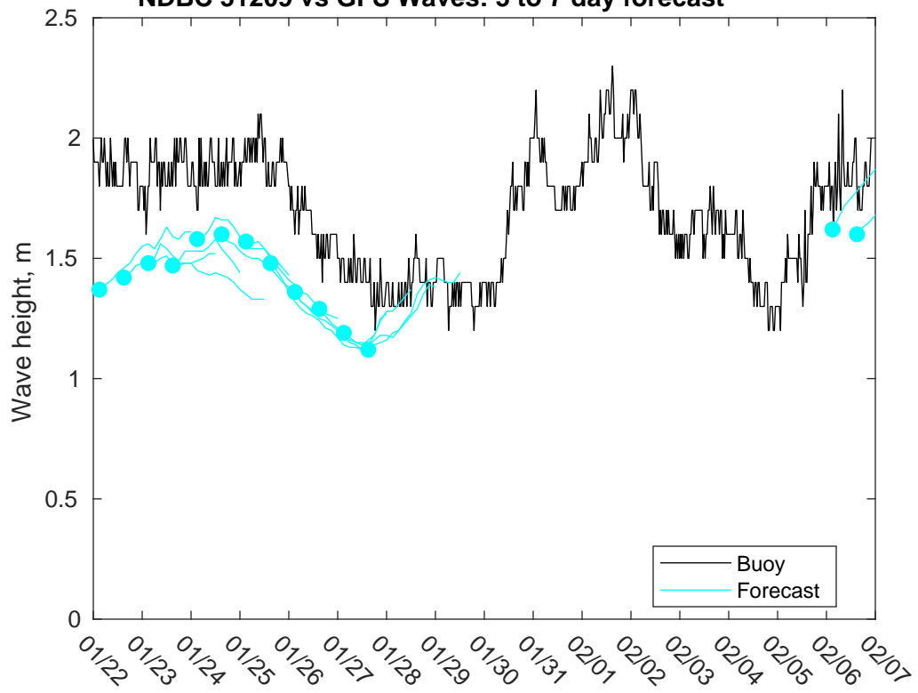
NDBC 51209 vs GFS Waves: 5 to 7 day forecast
