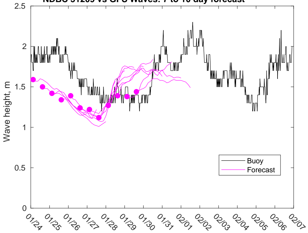
NDBC 51209 vs GFS Waves: 7 to 10 day forecast
