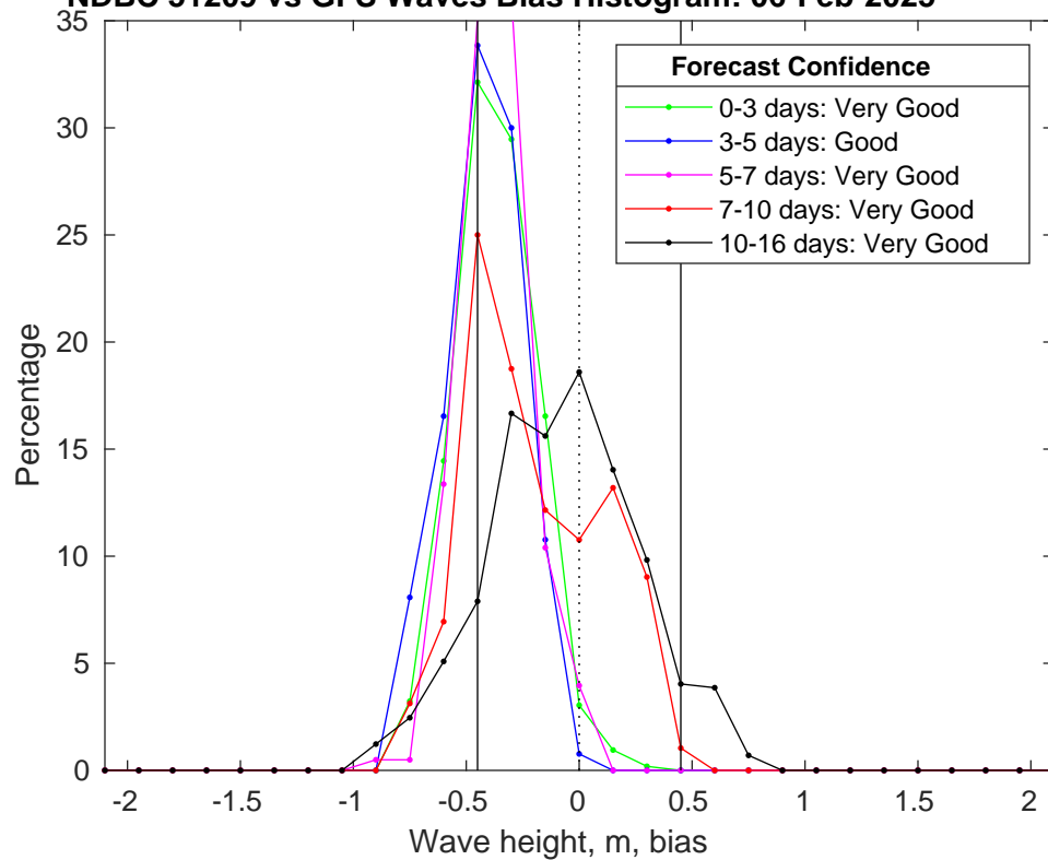
NDBC 51209 vs GFS Waves Bias Histogram: 06-Feb-2025
