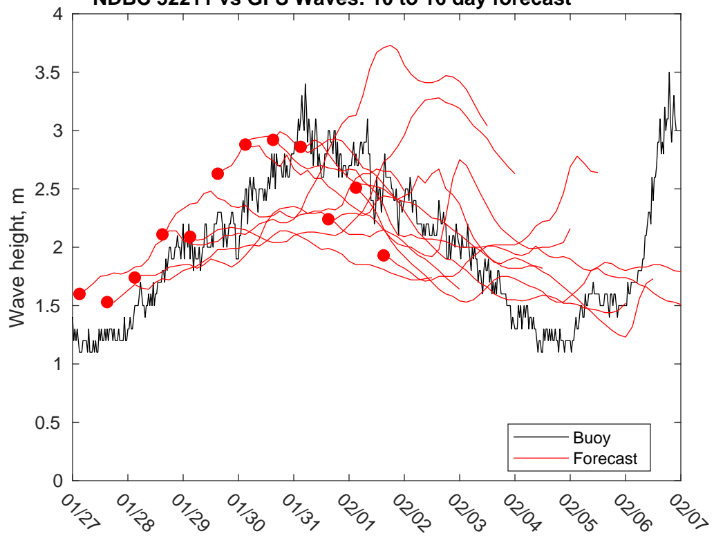
NDBC 52211 vs GFS Waves: 10 to 16 day forecast
