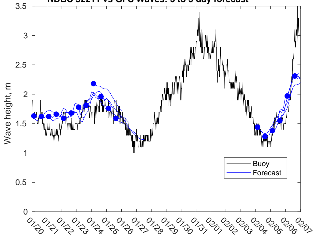
NDBC 52211 vs GFS Waves: 3 to 5 day forecast
