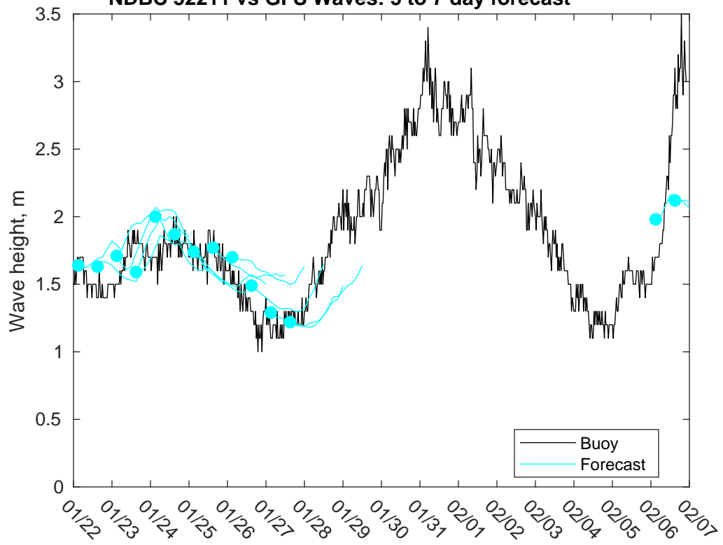
NDBC 52211 vs GFS Waves: 5 to 7 day forecast
