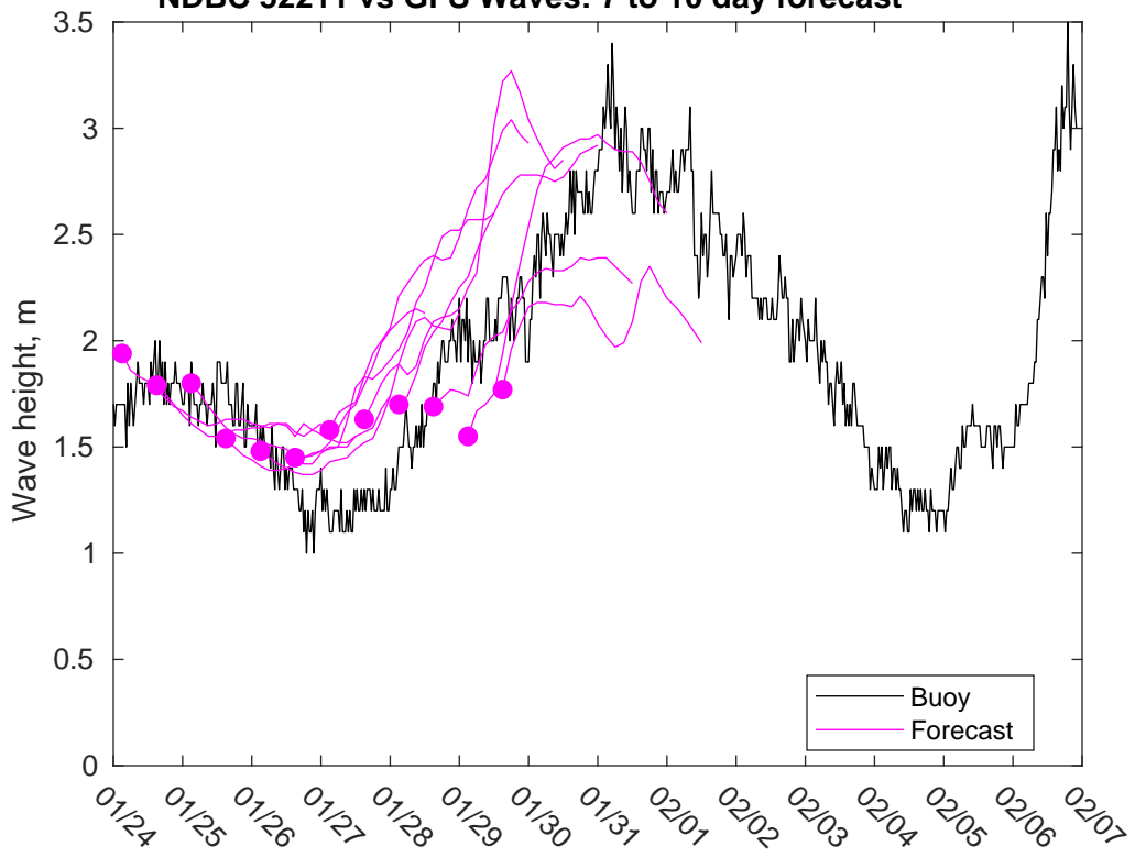
NDBC 52211 vs GFS Waves: 7 to 10 day forecast
