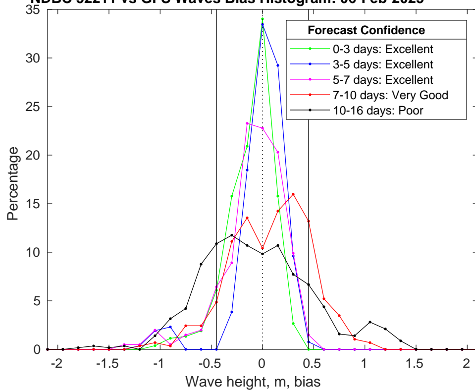
NDBC 52211 vs GFS Waves Bias Histogram: 06-Feb-2025
