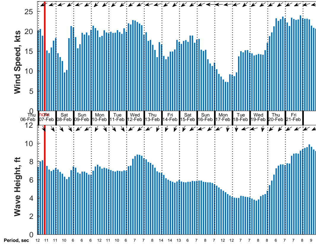
Wind & Wave Forecast for NDBC 52211 from 06-Feb-2025 22:00:00 to 22-Feb-2025 22:00:00
