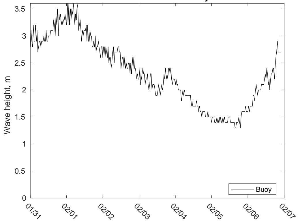
NDBC 52212 vs CMEMS Waves: 10 to 16 day forecast
