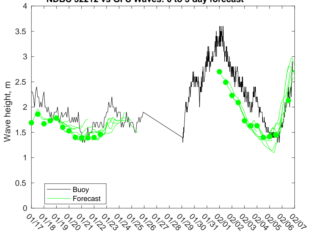
NDBC 52212 vs GFS Waves: 0 to 3 day forecast
