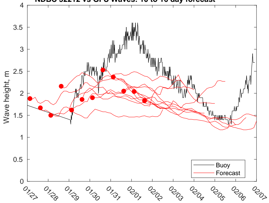
NDBC 52212 vs GFS Waves: 10 to 16 day forecast
