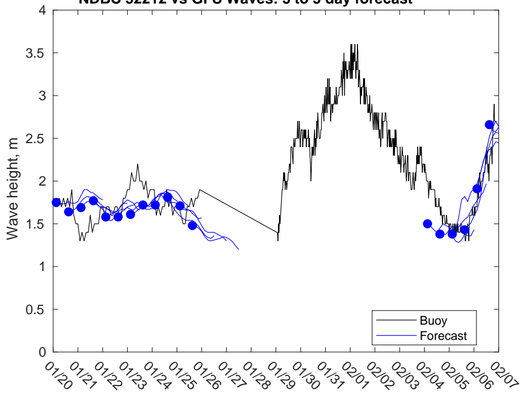
NDBC 52212 vs GFS Waves: 3 to 5 day forecast
