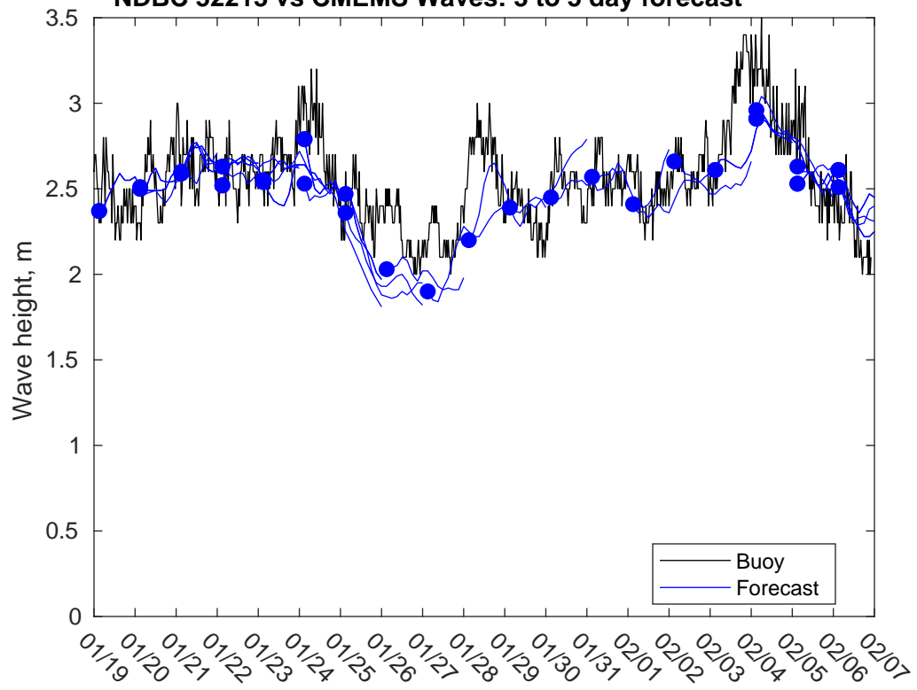
NDBC 52213 vs CMEMS Waves: 3 to 5 day forecast
