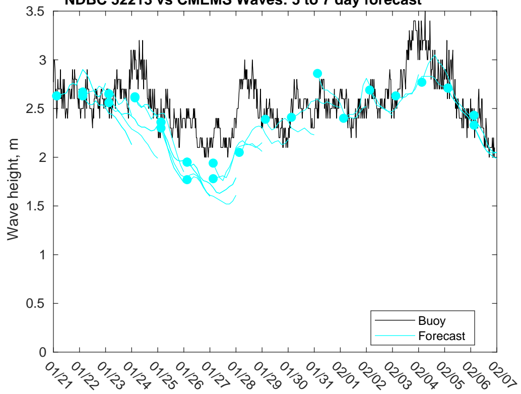
NDBC 52213 vs CMEMS Waves: 5 to 7 day forecast
