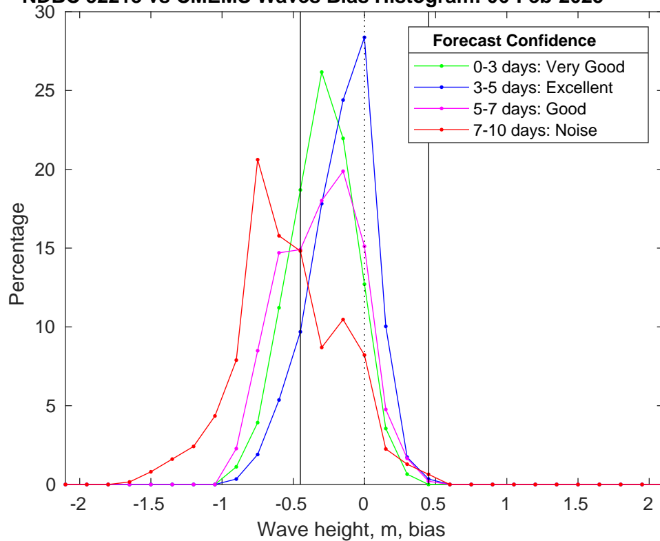
NDBC 52213 vs CMEMS Waves Bias Histogram: 06-Feb-2025
