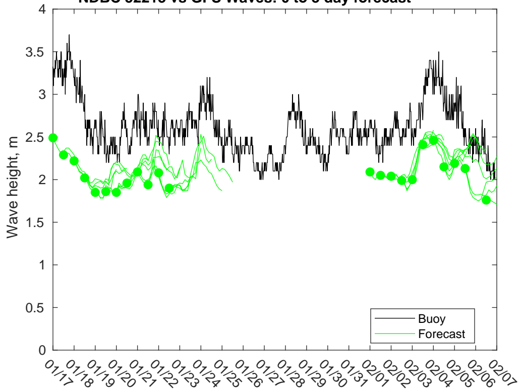
NDBC 52213 vs GFS Waves: 0 to 3 day forecast
