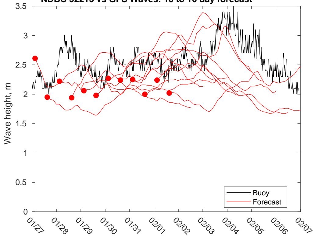
NDBC 52213 vs GFS Waves: 10 to 16 day forecast
