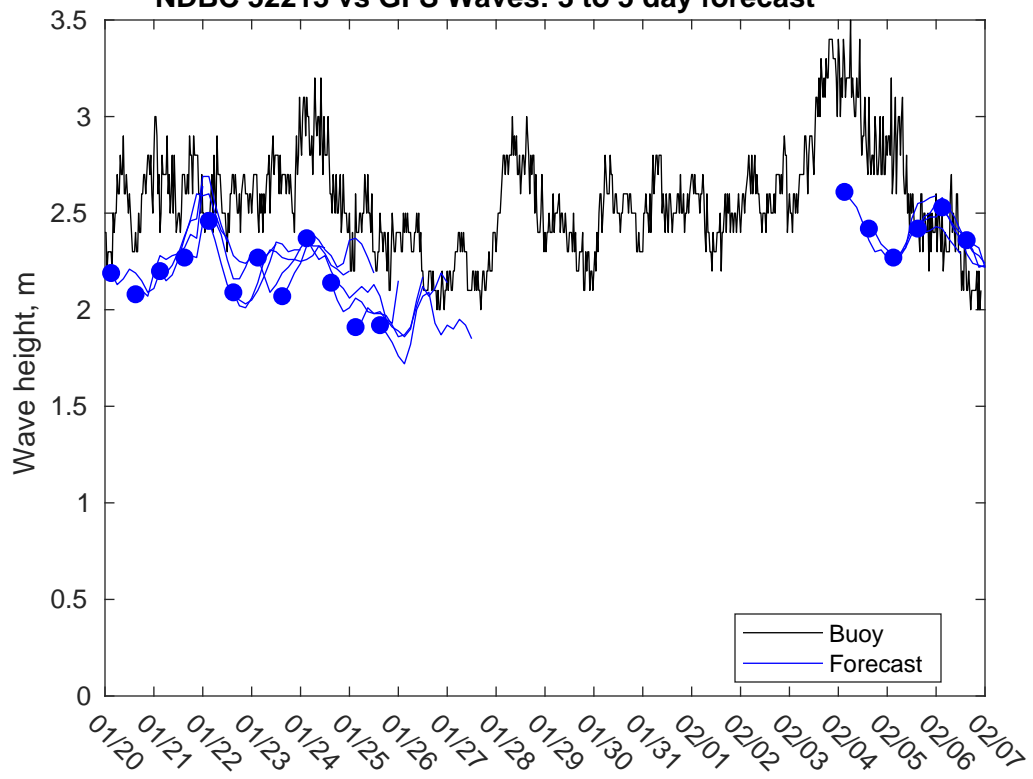
NDBC 52213 vs GFS Waves: 3 to 5 day forecast
