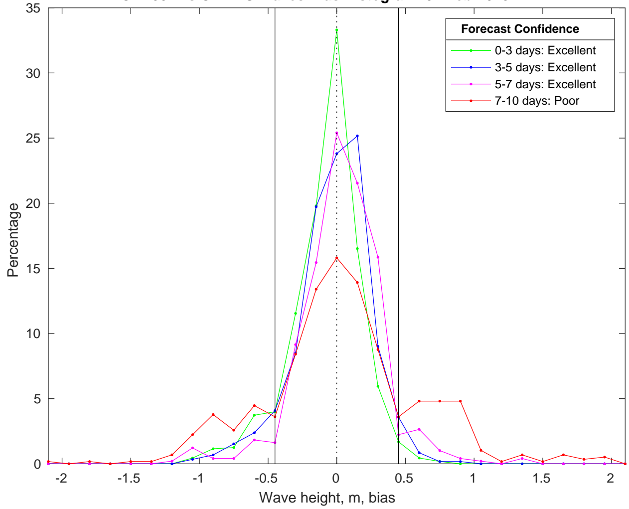
NDBC 41004 vs CMEMS Waves Bias Histogram: 07-Feb-2025
