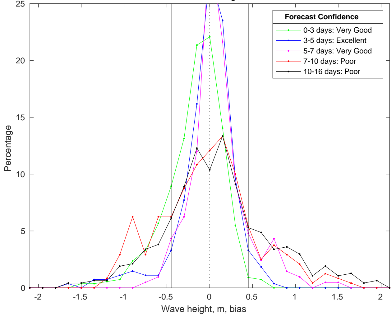
NDBC 41004 vs GFS Waves Bias Histogram: 07-Feb-2025
