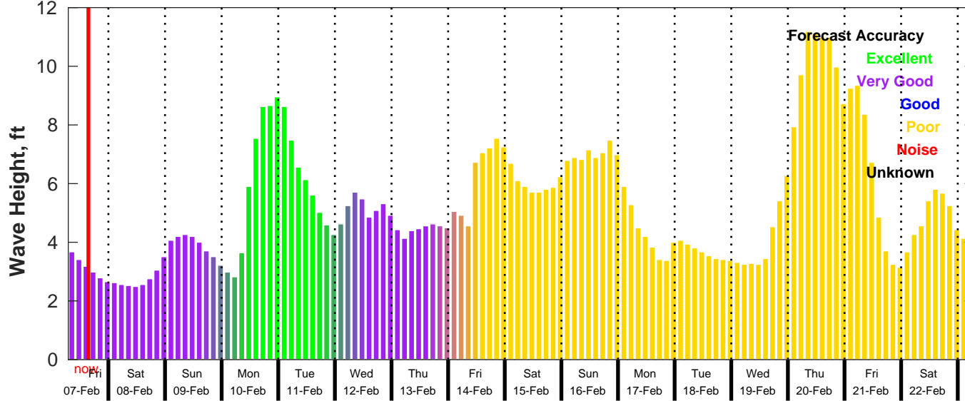
GFS Wave Forecast for NDBC 41004 from 07-Feb-2025 07:00:00 to 23-Feb-2025 07:00:00
